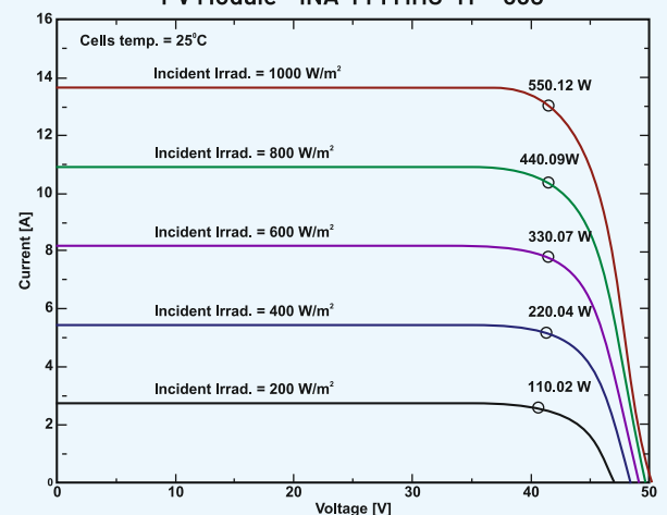
I-V Characteristics at Different Irradiance PV Module - INA-144 MHC-TF - 550
