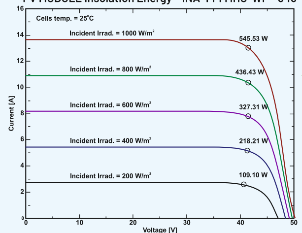
I-V CHARACTERISTICS AT DIFFERENT IRRADIANCE PV MODULE Insolation Energy - INA-144 MHC-WF - 545
